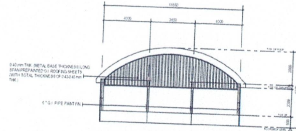
2 REAR SIDE ELEVATION SCALE 1 : 100 MTS
